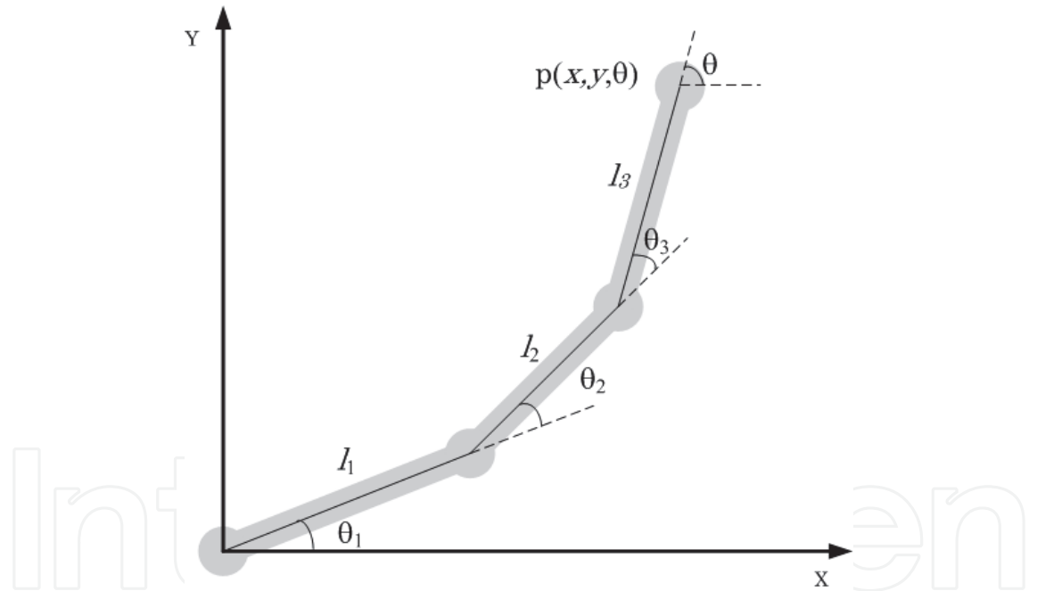
Fig. 6. Geometric of three link planar robot
